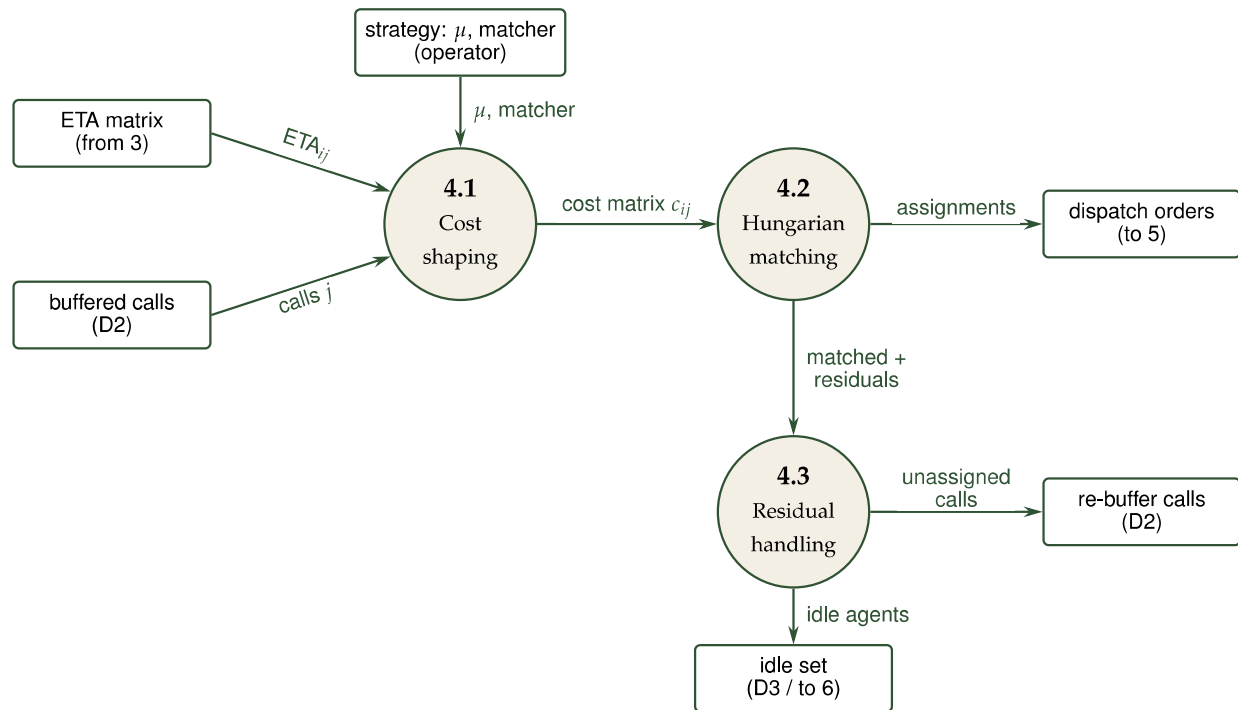
Figure 3: Level 2 — Process 4 (Batch Assignment). Deconstruction of cost shaping, matching, and residual set partitioning.
