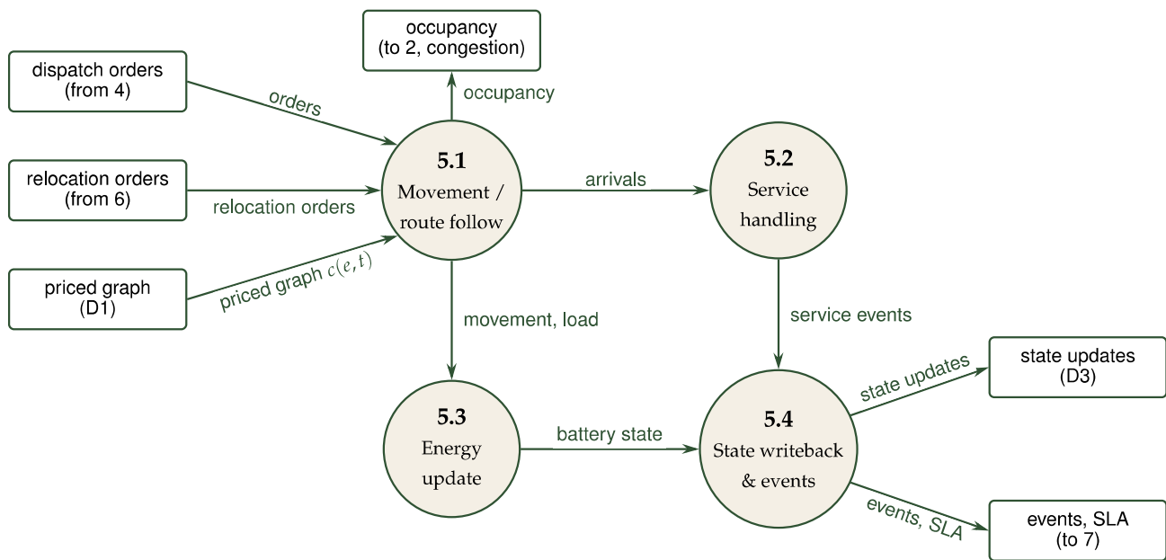
Figure 4: Level 2 — Process 5 (Agent Execution). Internal agent simulation pipeline with dedicated entry/exit corridors and decoupled congestion telemetry.
